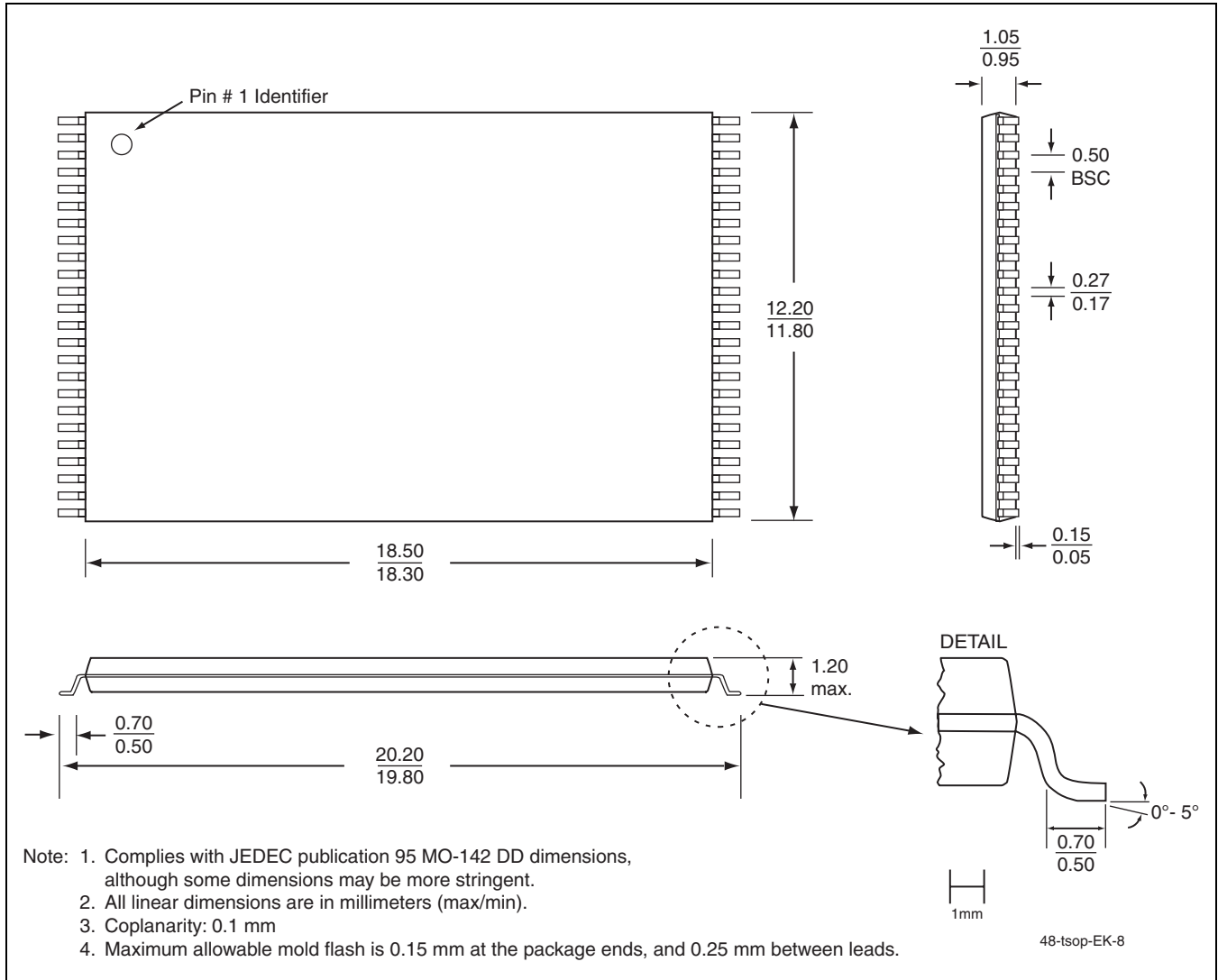
FIGURE 21: 48-Lead Thin Small Outline Package (TSOP) 12mm x 20mm SST Package Code: EK
