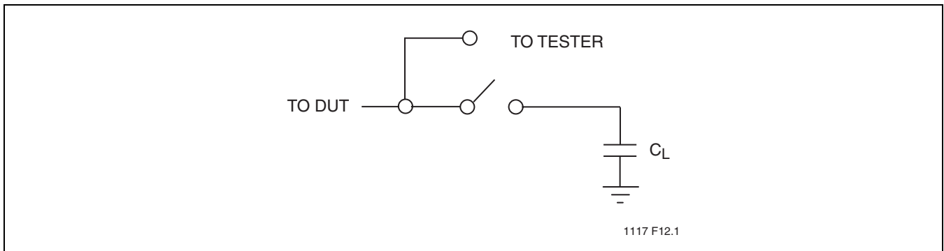
FIGURE 16: A Test Load Example
