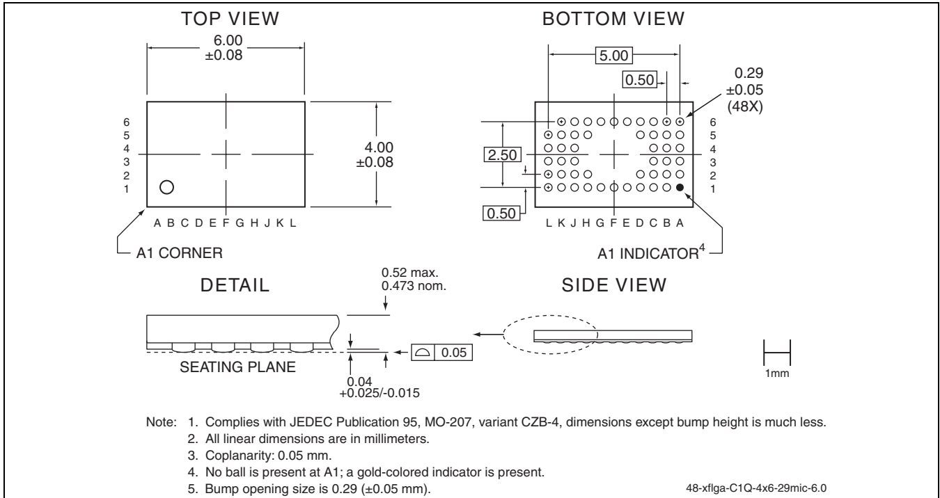
FIGURE 24: 48-Bump Extremely-Thin-Profile, Fine-Pitch Land Grid Array (XFLGA) 4mm x 6mm SST Package Code: C1Q
