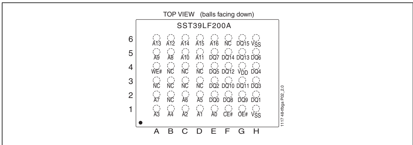
FIGURE 3: Pin Assignments for 48-Ball TFBGA
