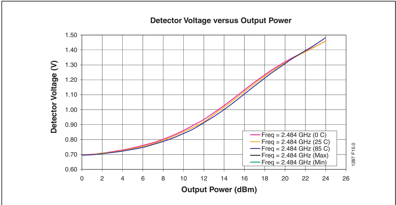
FIGURE 15: Low Band CH14 Detector Characteristics over Temperature with 2:1 Output VSWR All Phases
