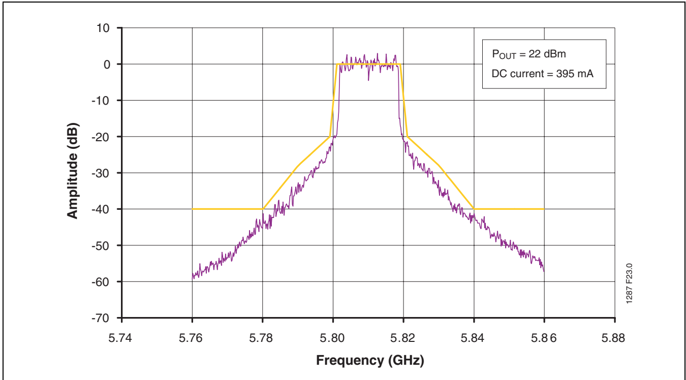
FIGURE 24: High Band 802.11a Spectrum Mask at 5.805 GHz at Output Power 22 dBm with DC Current at 395 mA
