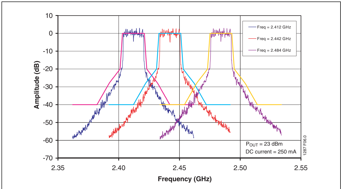
FIGURE 7: Low Band 802.11g Spectrum Mask at 23 dBm with DC Current at 250 mA
