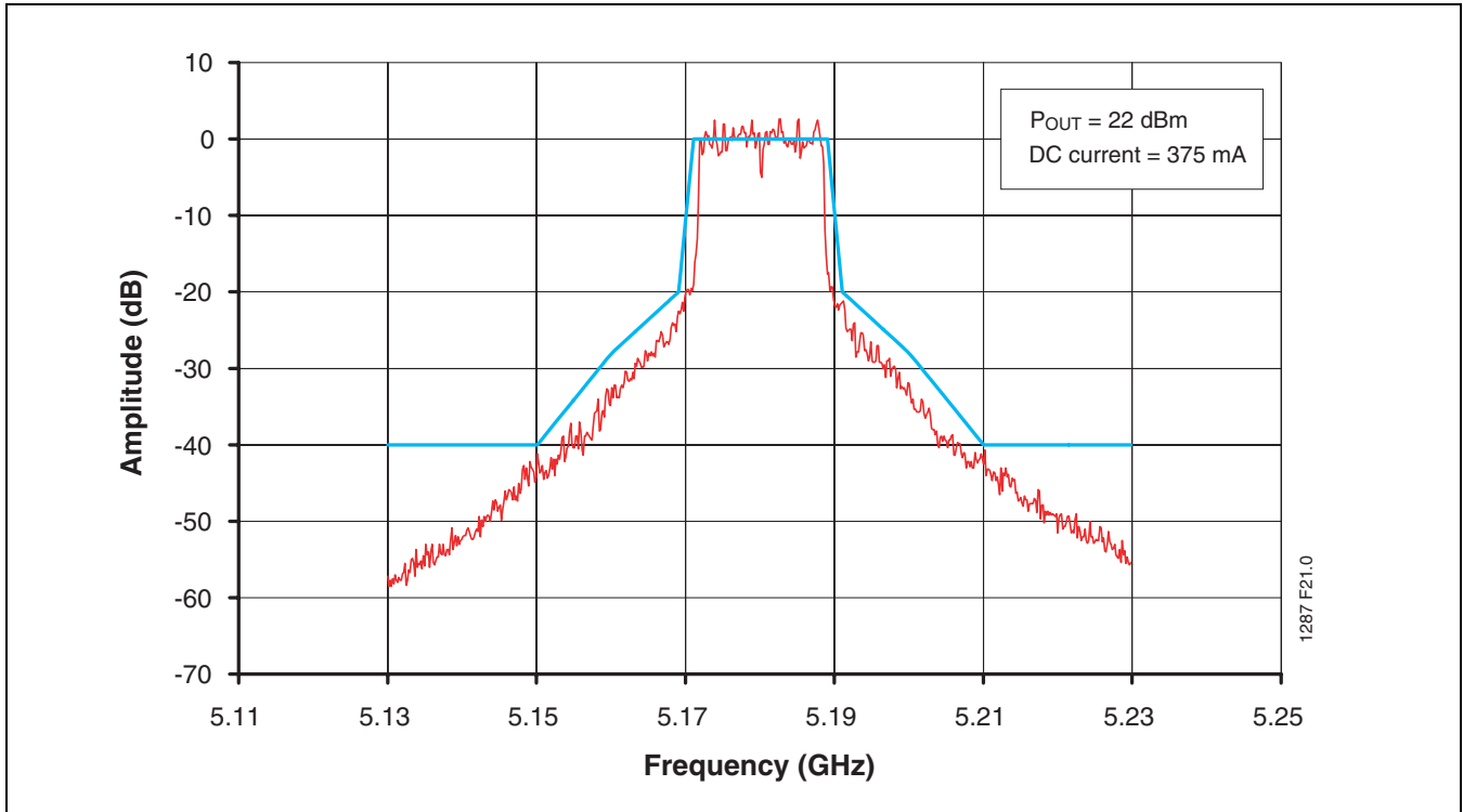
FIGURE 22: High Band 802.11a Spectrum Mask at 5.18 GHz at Output Power 22 dBm with DC Current at 375 mA
