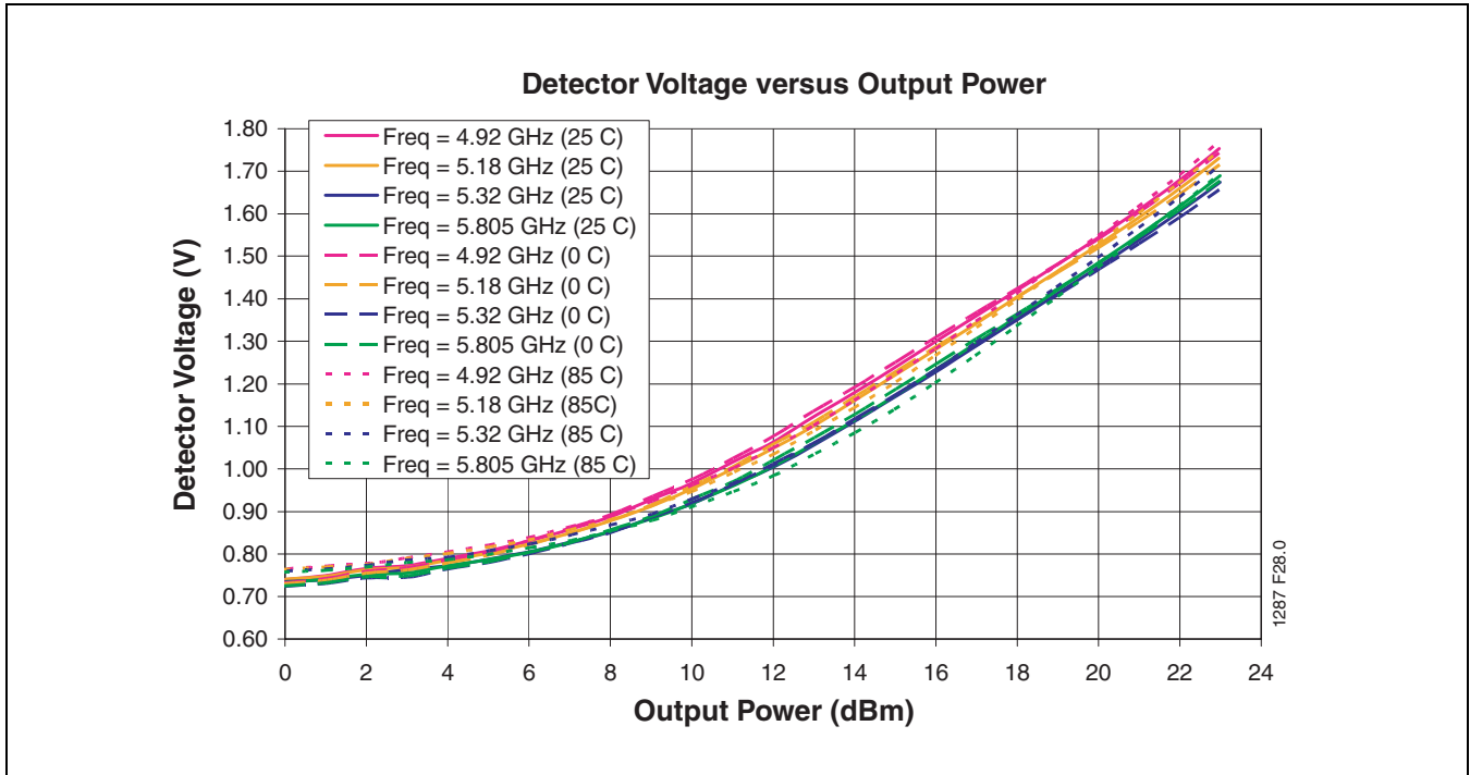
FIGURE 29: High Band Detector Characteristics over Temperature and over Frequency
