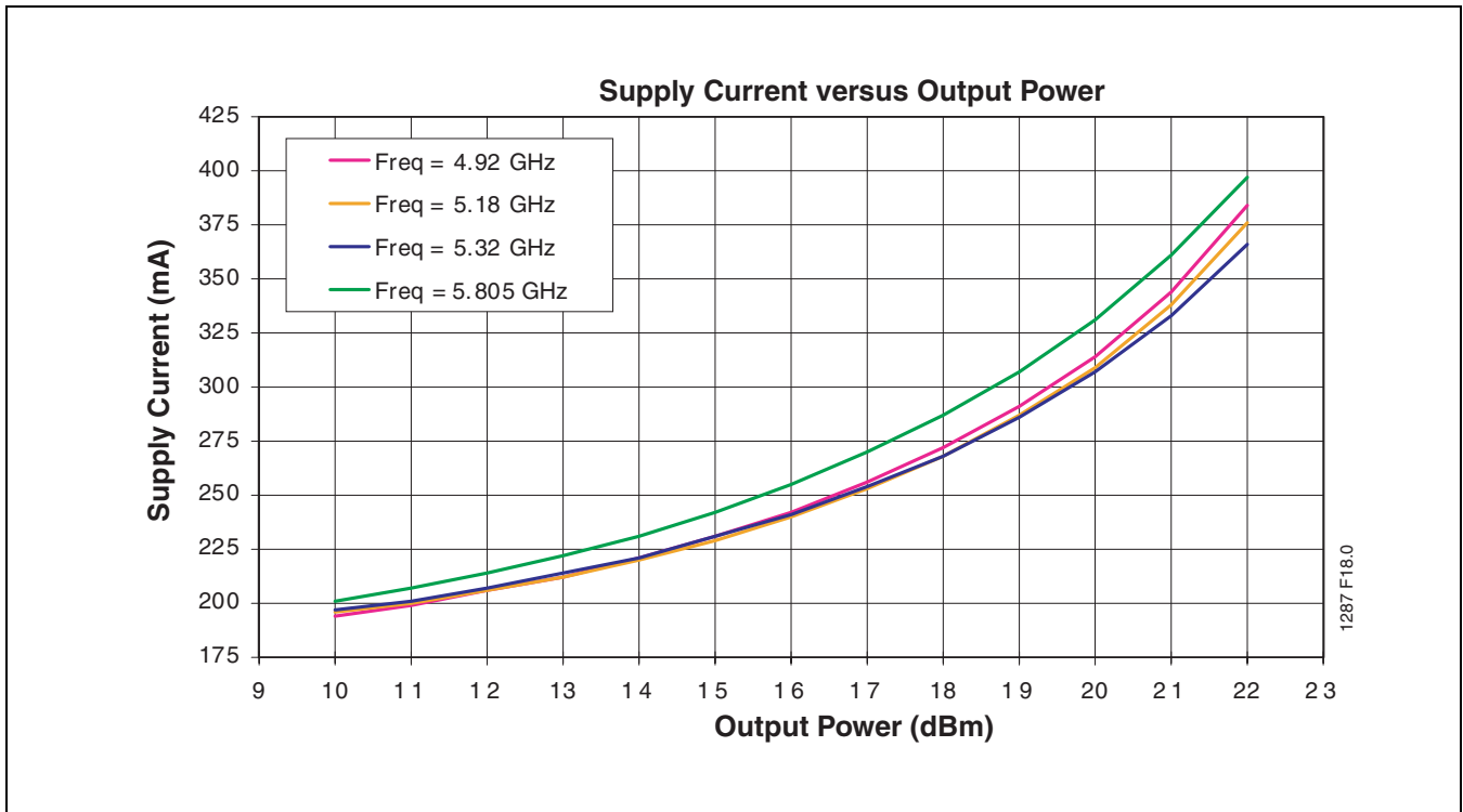
FIGURE 19: High Band Power Supply Current versus Output Power
