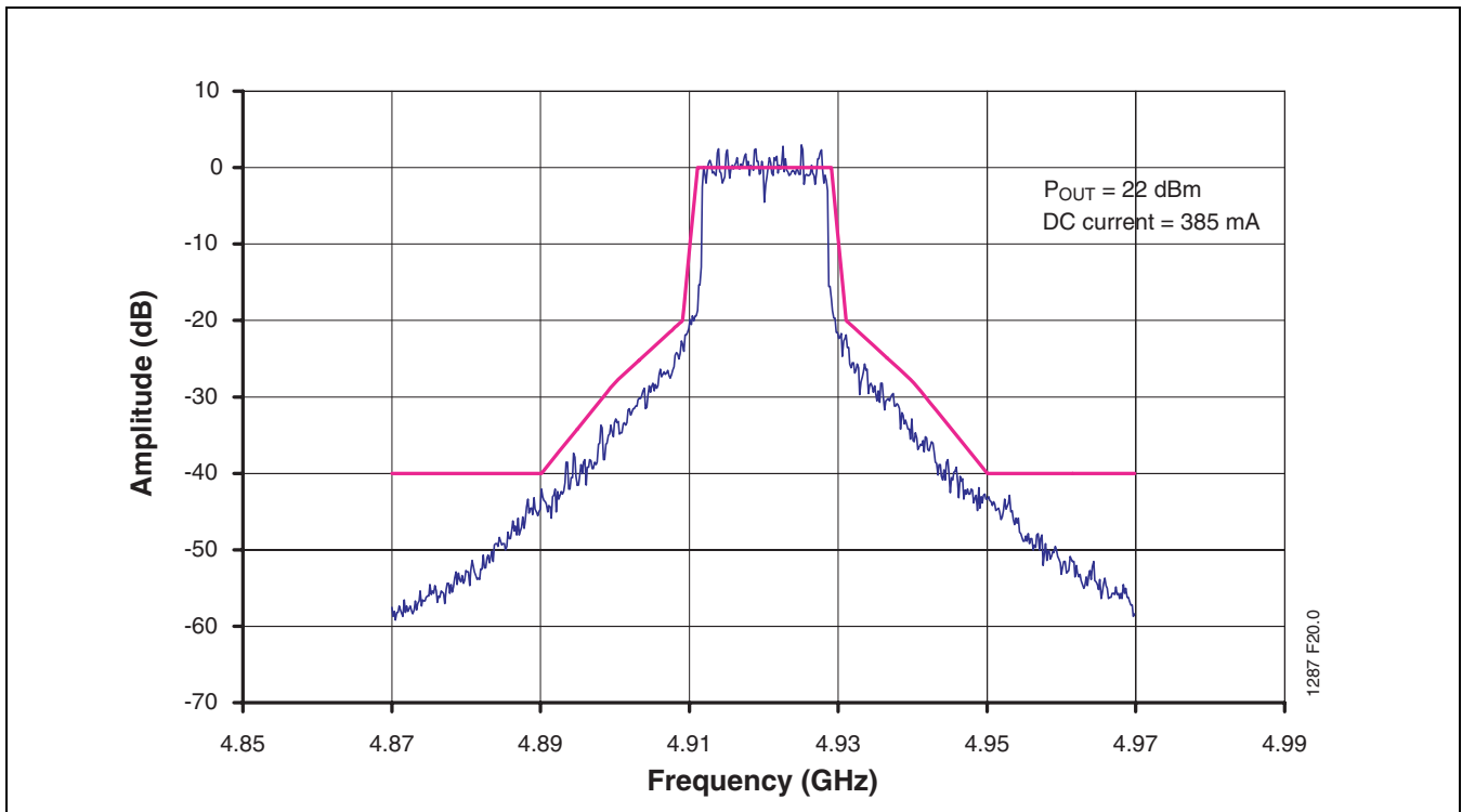
FIGURE 21: High Band 802.11a Spectrum Mask at 4.92 GHz at Output Power 22 dBm with DC Current at 385 mA
