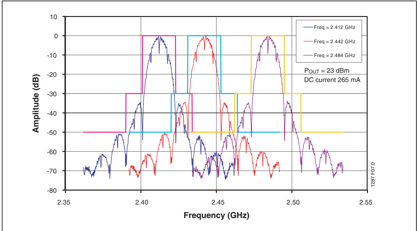
FIGURE 8: Low Band 802.11b Spectrum Mask at 23 dBm with DC Current of 265 mA
