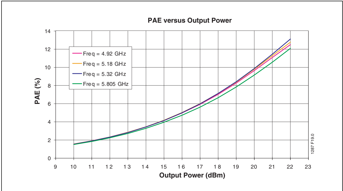
FIGURE 20: High Band PAE versus Output Power
