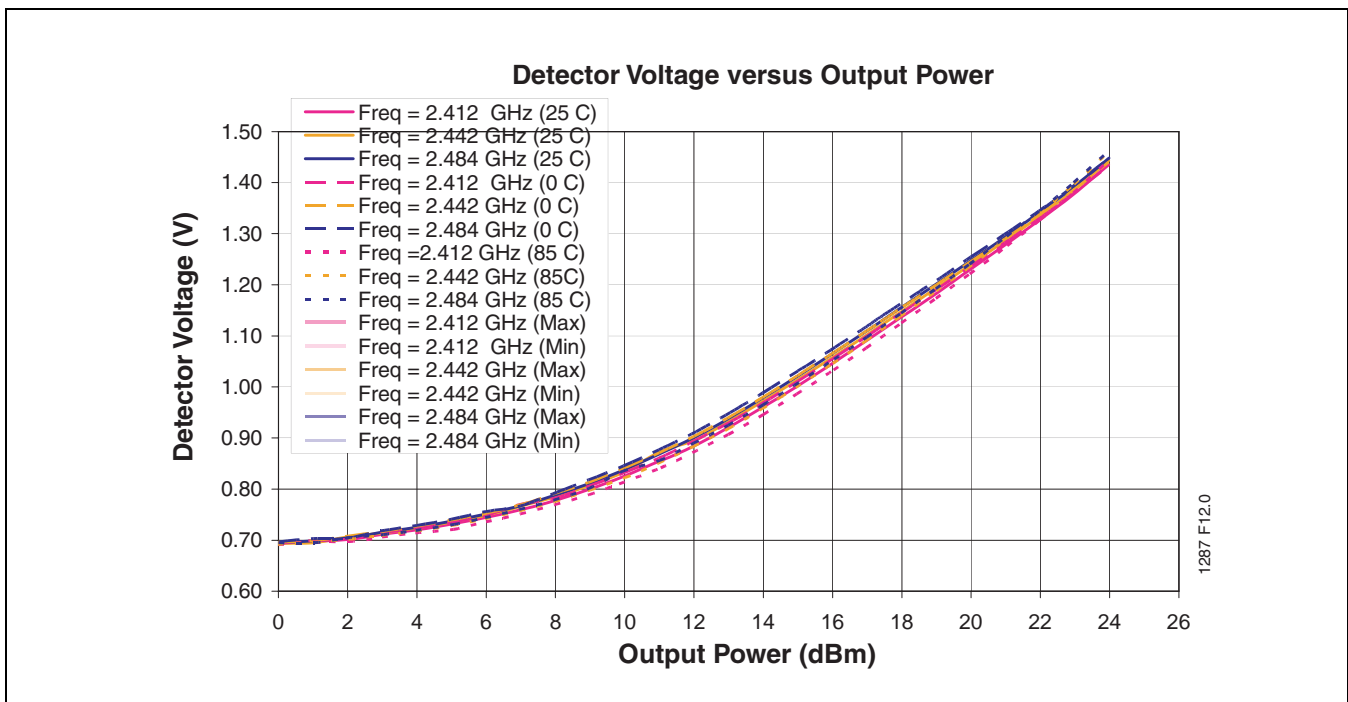
FIGURE 12: Low Band Detector Characteristics over Temperature with 2:1 Output VSWR All Phases
