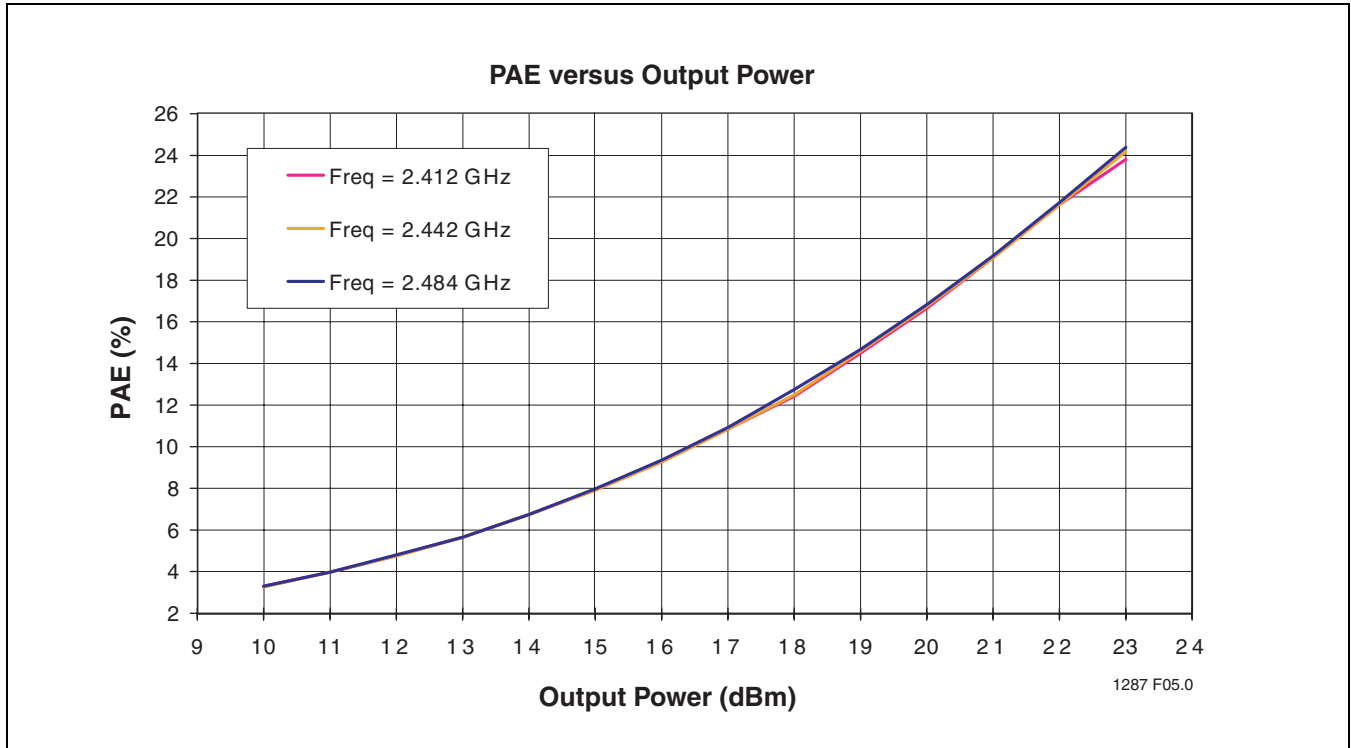
FIGURE 6: Low BAnd PAE versus Output Power
