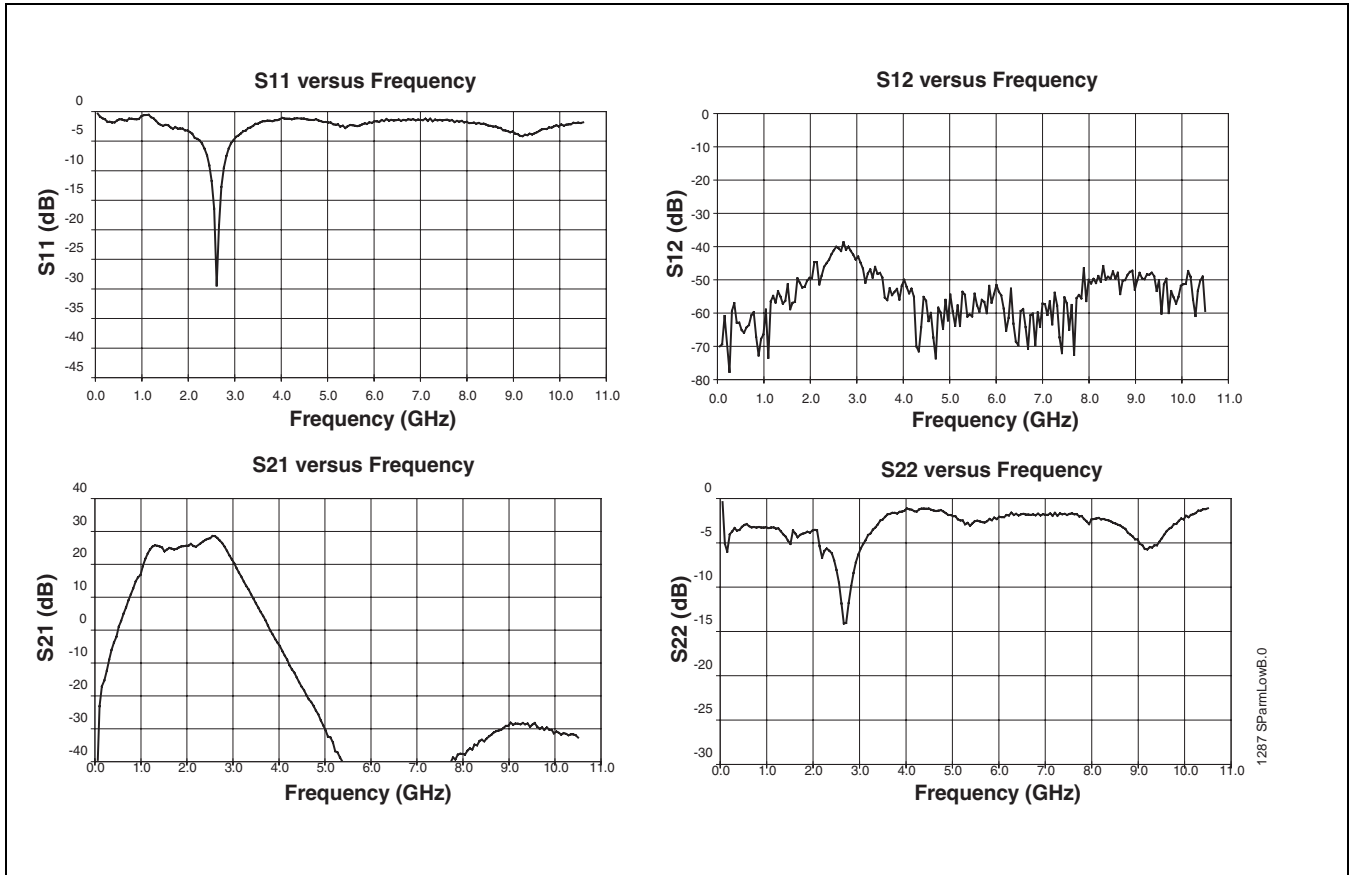
FIGURE 3: Low Band S-Parameters
