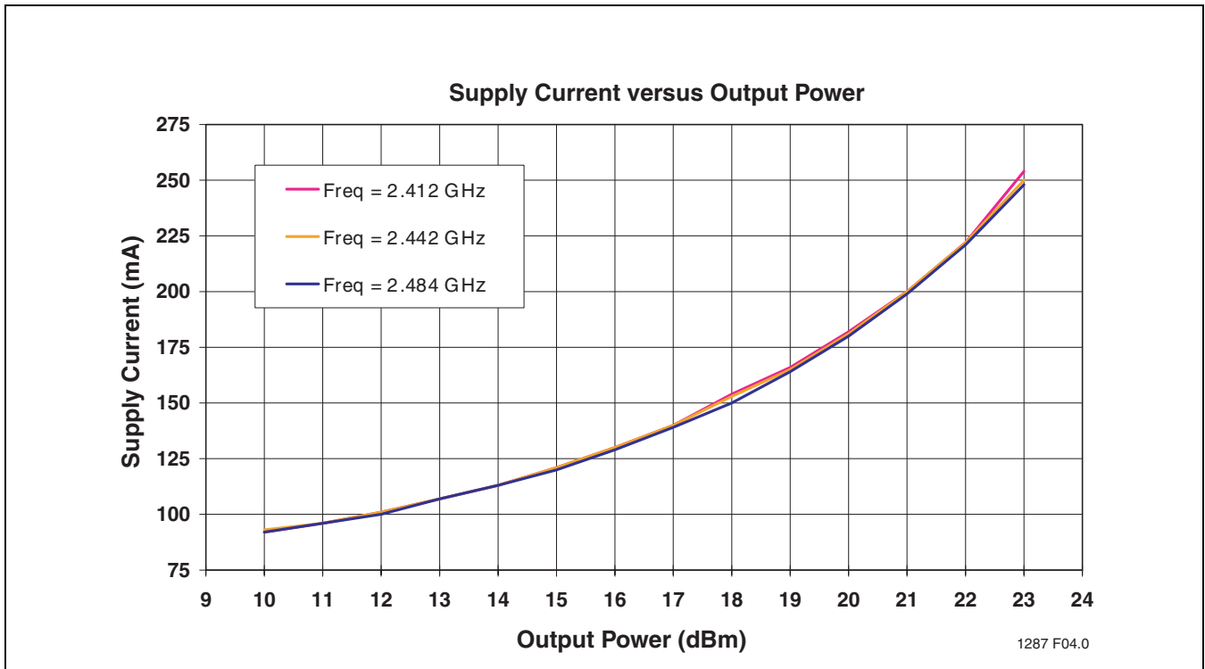
FIGURE 5: Low Band Power Supply Current versus Output Power
