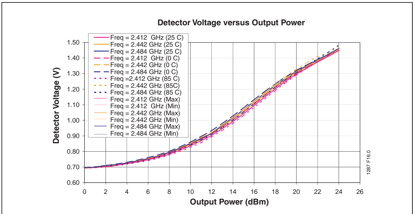
FIGURE 16: Low Band Detector Characteristics over Temperature with 2:1 Output VSWR All Phases
