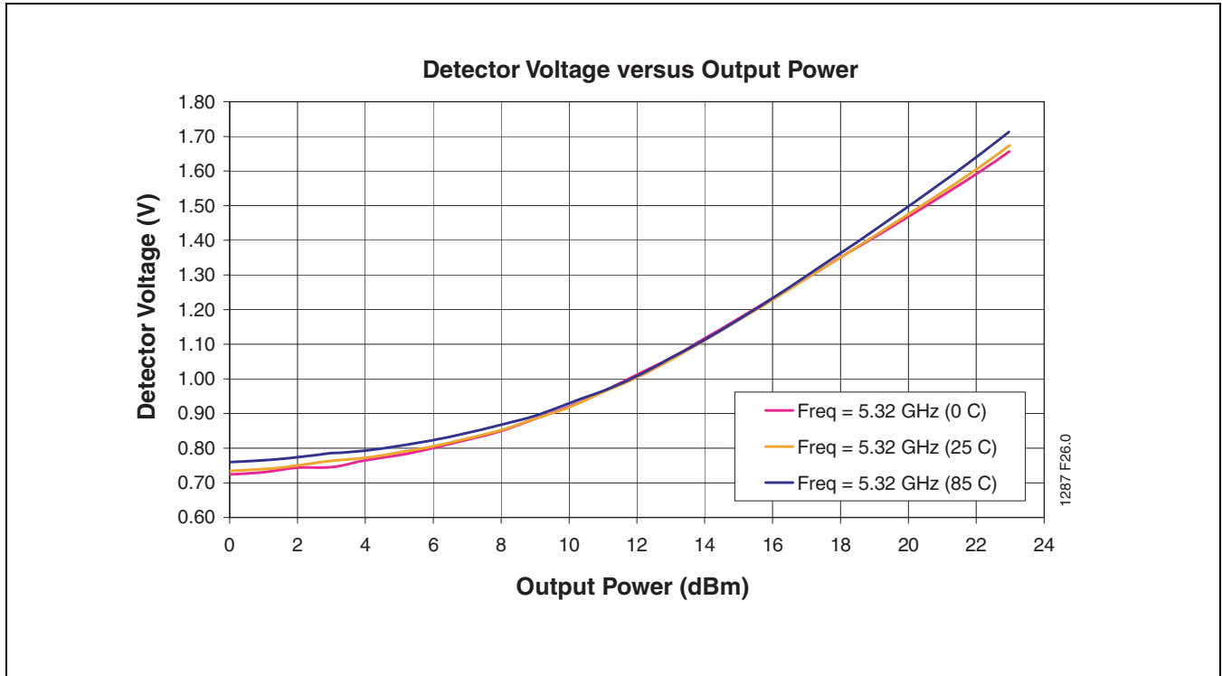
FIGURE 27: High Band Detector Characteristics over Temperature at 5.32 GHz
