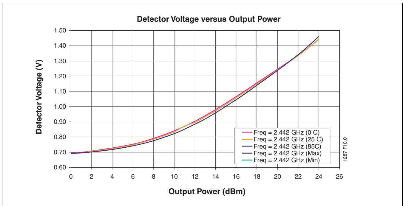
FIGURE 10: Low Band CH7 Detector Characteristics over Temperature with 2:1 Output VSWR All Phases
