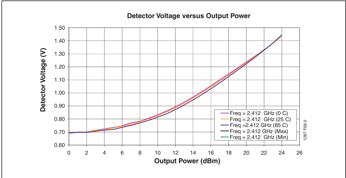
FIGURE 9: Low Band CH1 Detector Characteristics over Temperature with 2:1 Output VSWR All Phases
