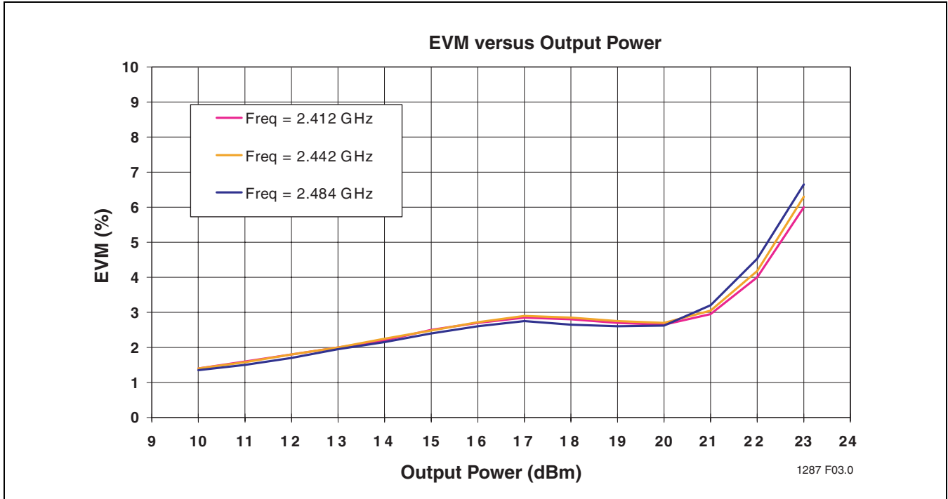
FIGURE 4: Low Band EVM versus Output Power
