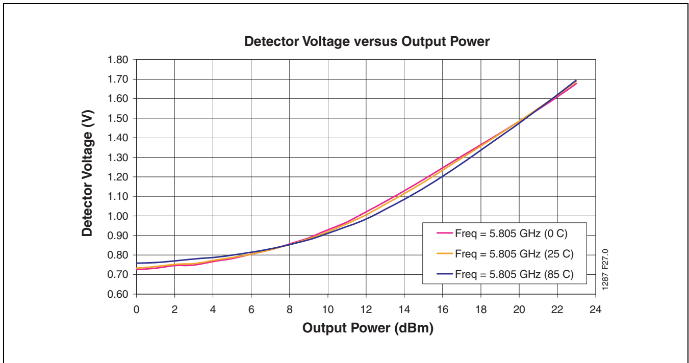
FIGURE 28: High Band Detector Characteristics over Temperature at 5.805 GHz
