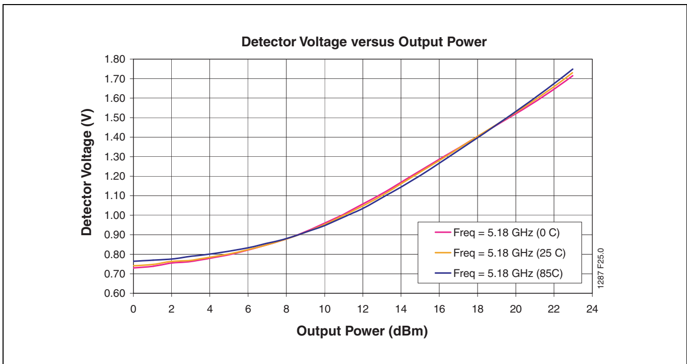
FIGURE 26: High Band Detector Characteristics over Temperature at 5.18 GHz
