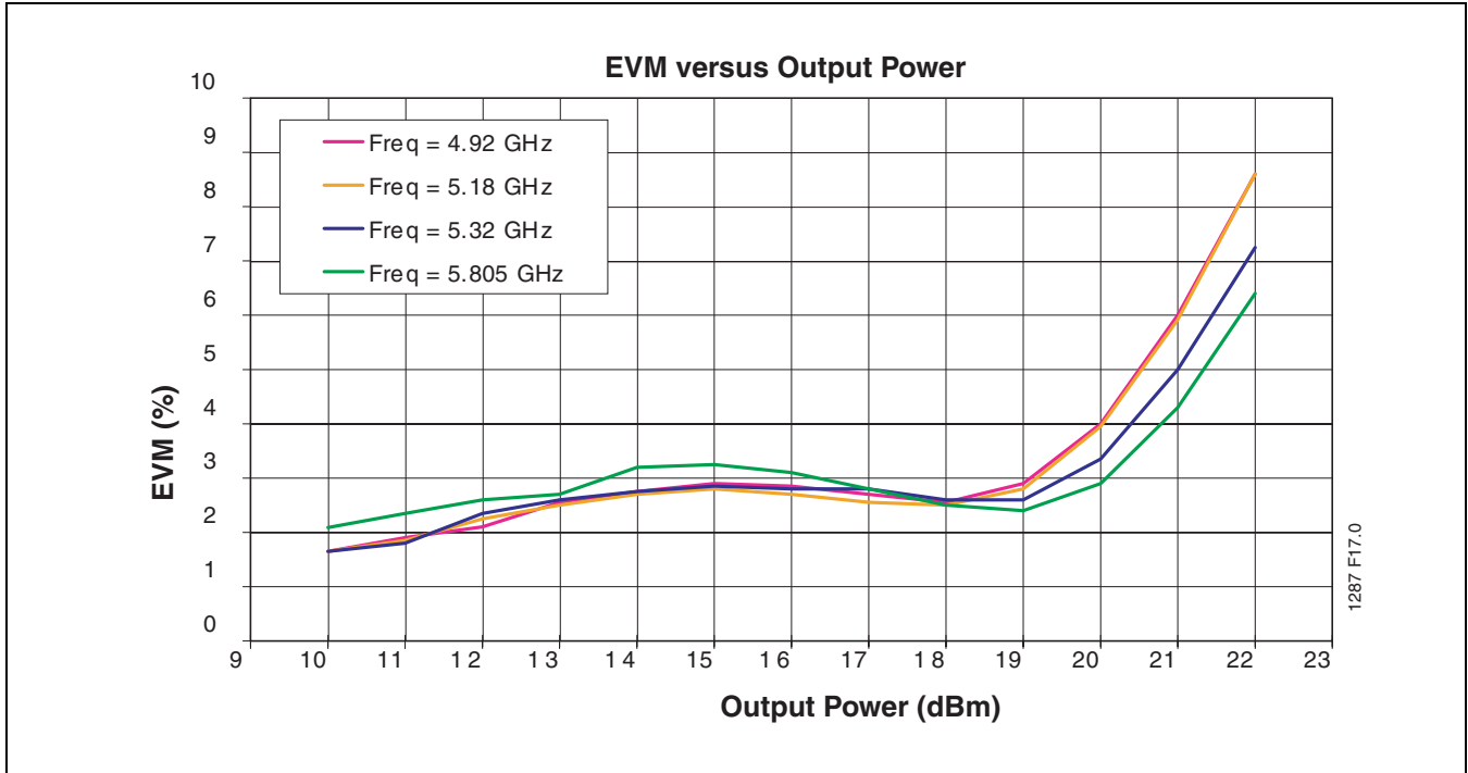
FIGURE 18: High Band EVM versus Output Power
