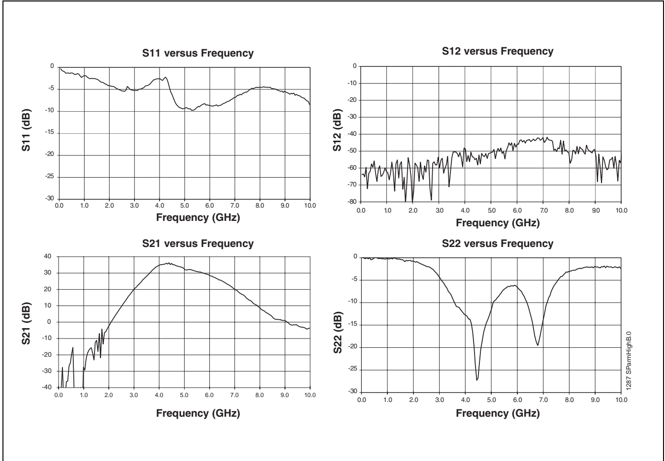
FIGURE 17: High Band S-Parameters
