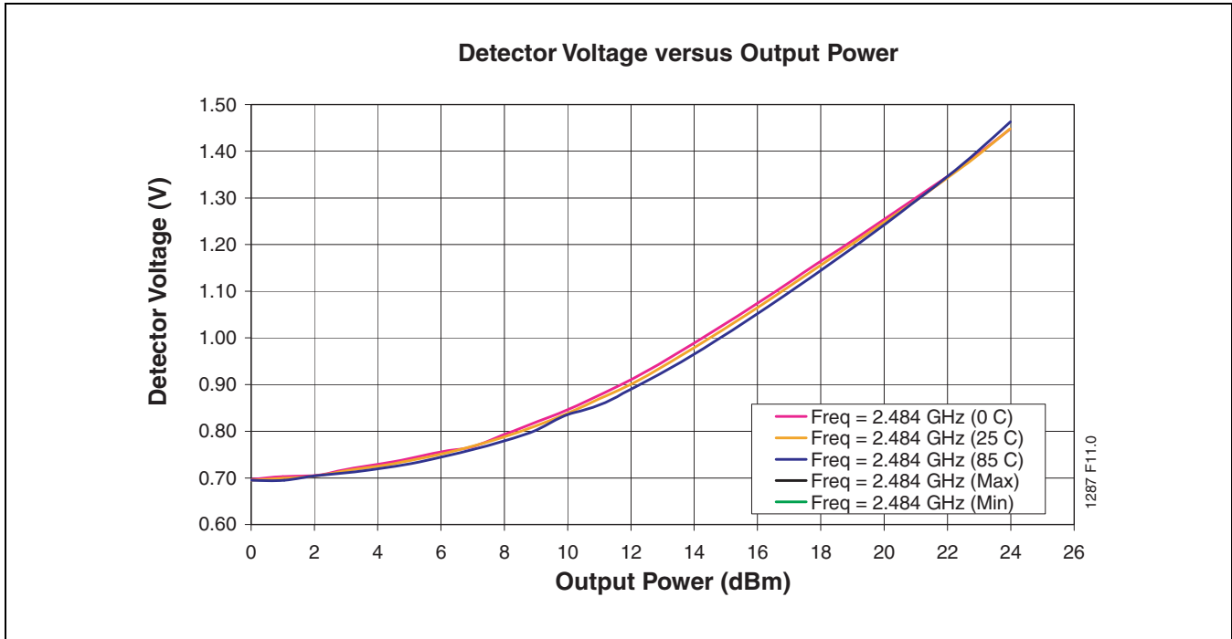
FIGURE 11: Low Band CH14 Detector Characteristics over Temperature with 2:1 Output VSWR All Phases
