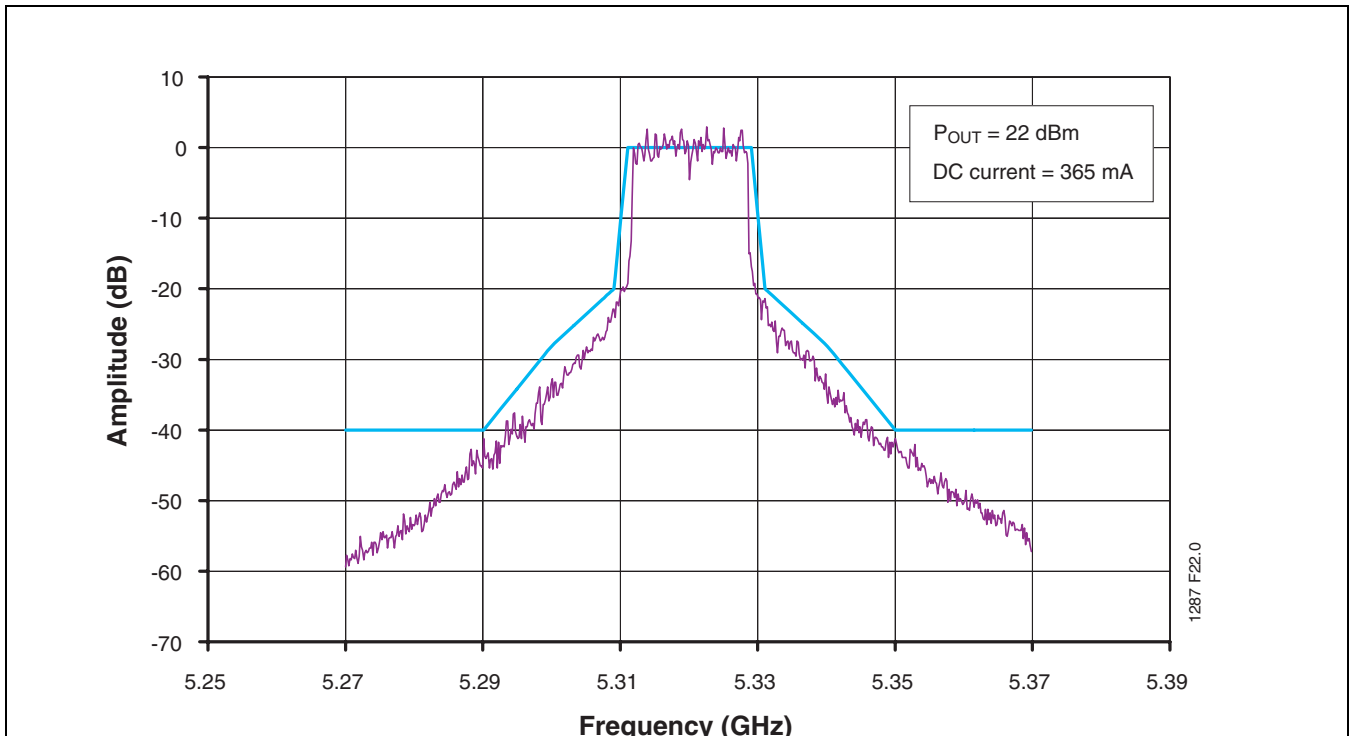
FIGURE 23: High Band 802.11a Spectrum Mask at 5.32 GHz at Output Power 22 dBm with DC Current at 365 mA
