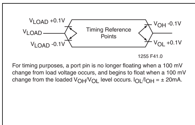
FIGURE 14-9: Float Waveform
