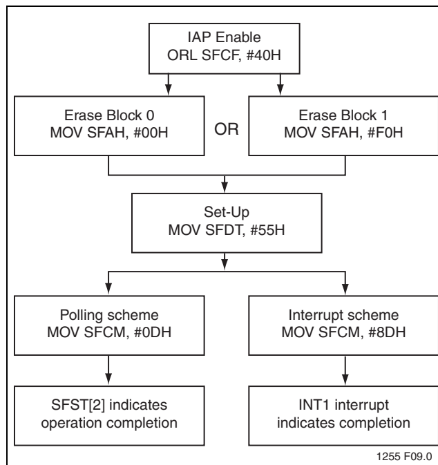
FIGURE 4-2: Block-Erase
