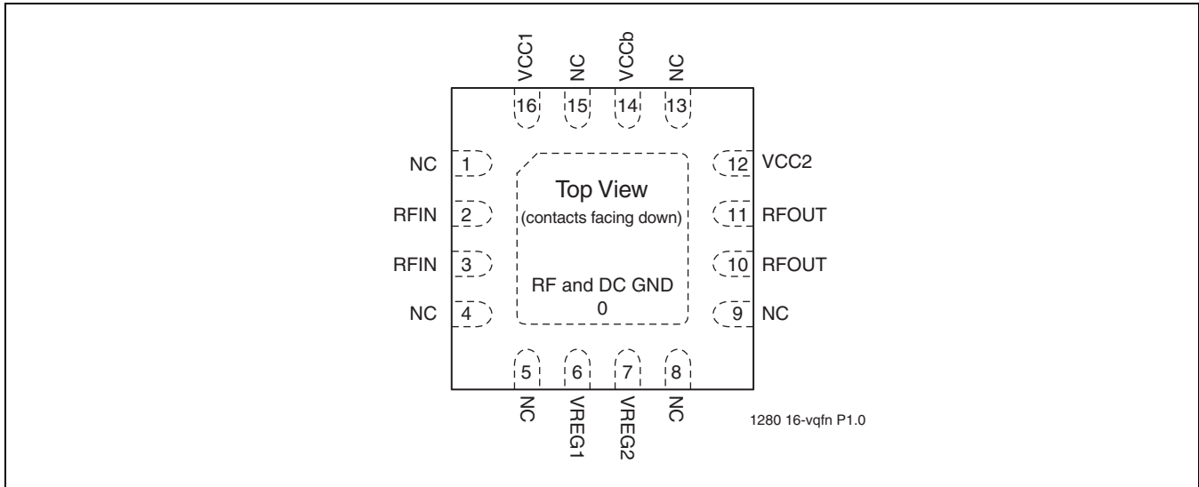
FIGURE 1: PIN ASSIGNMENTS FOR 16-CONTACT VQFN
