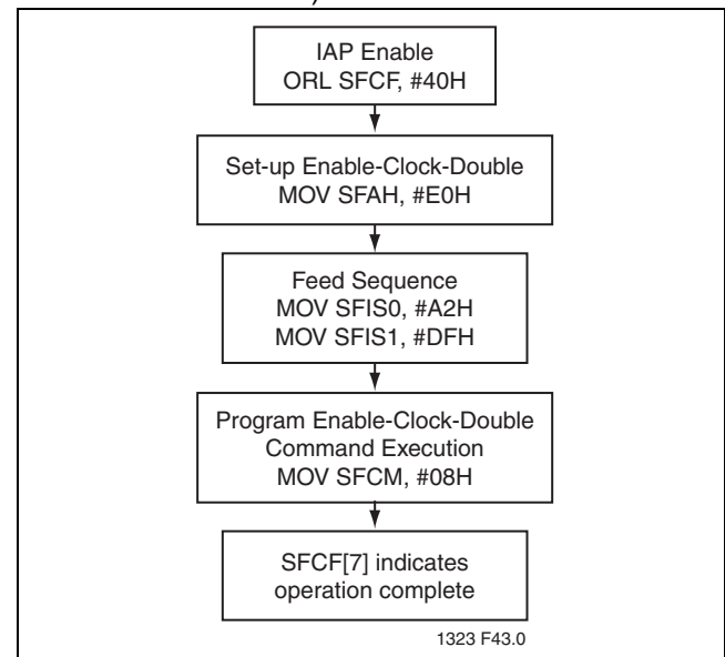
FIGURE 4-7: Enable-Clock-Double
