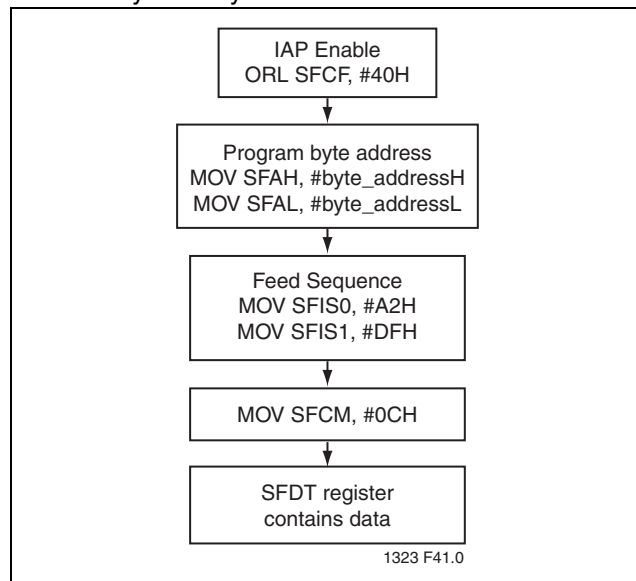
FIGURE 4-5: Byte-Verify
