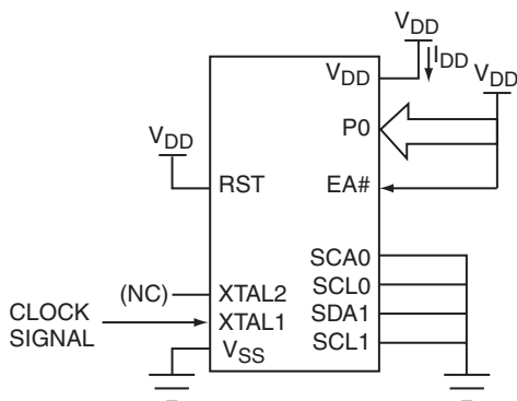
FIGURE 12-8: I_{DD} Test Condition, Active Mode
