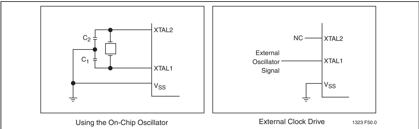
FIGURE 11-1: Oscillator Characteristics
