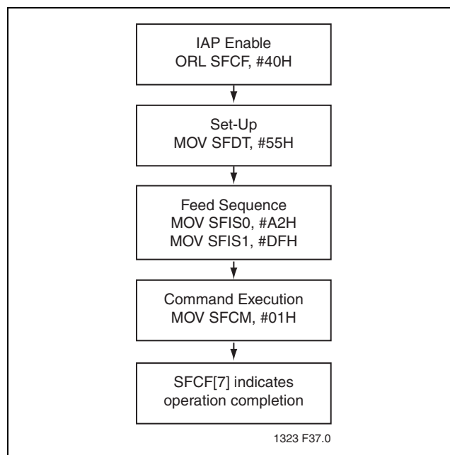
FIGURE 4-1: Chip-Erase
