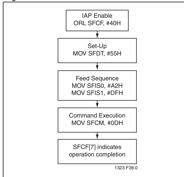
FIGURE 4-2: Partition0-Erase
