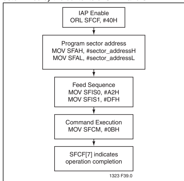
FIGURE 4-3: Sector-Erase
