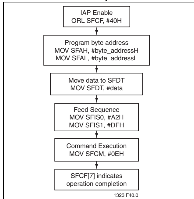
FIGURE 4-4: Byte-Program
