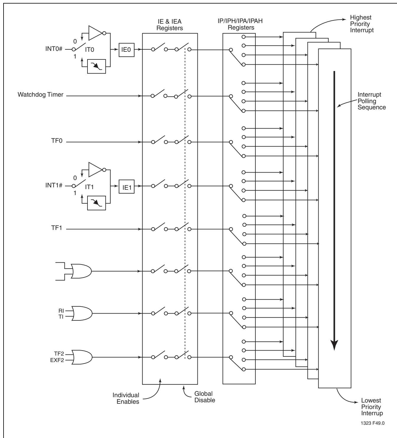
FIGURE 9-2: Interrupt Sequence
