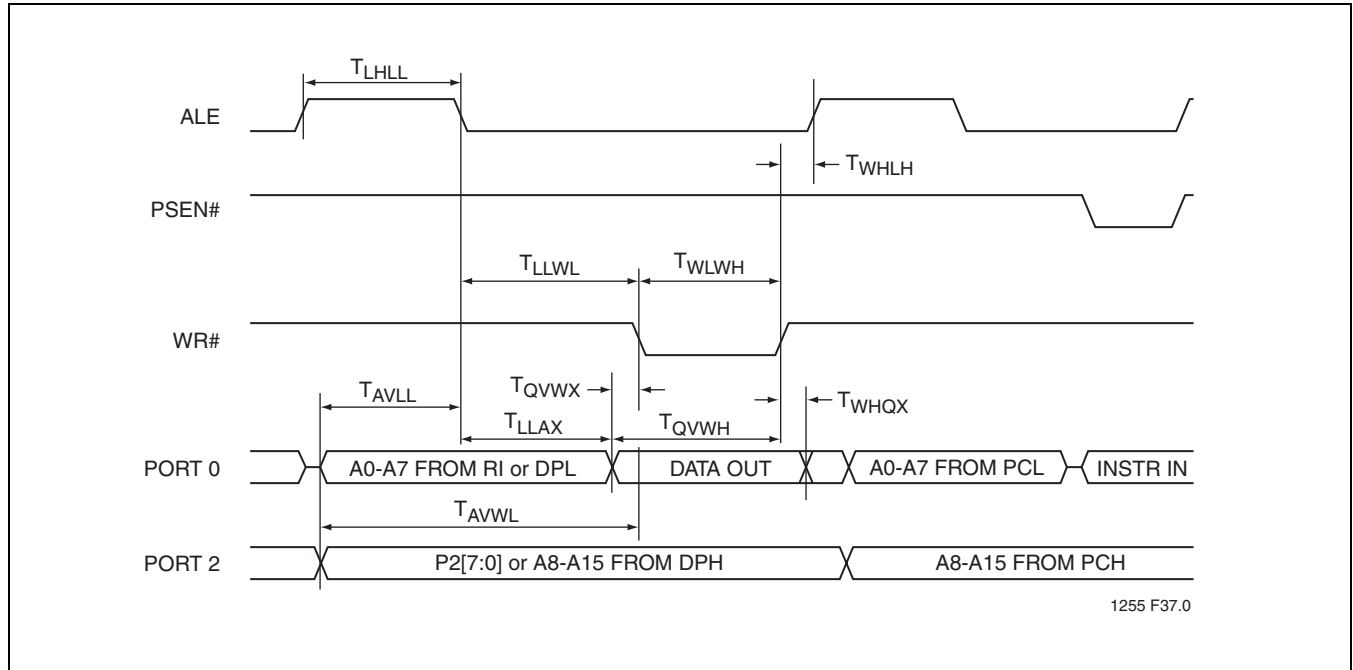
FIGURE 14-4: External Data Memory Write Cycle
