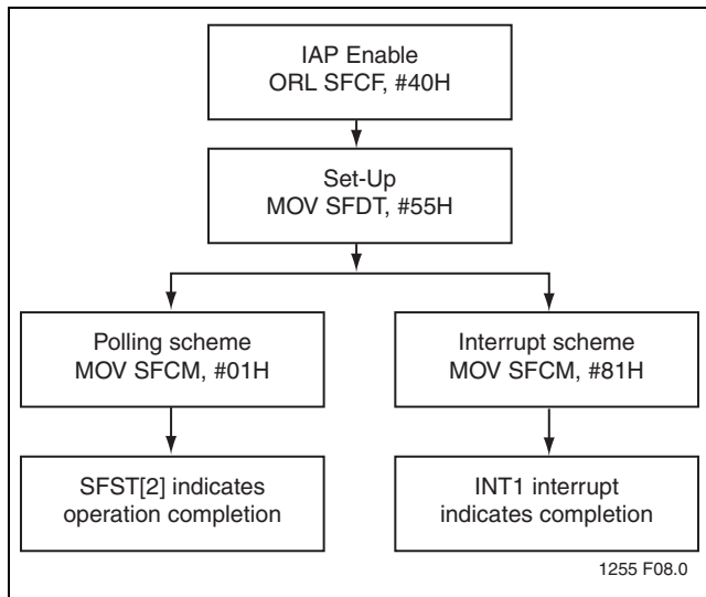
FIGURE 4-1: Chip-Erase
