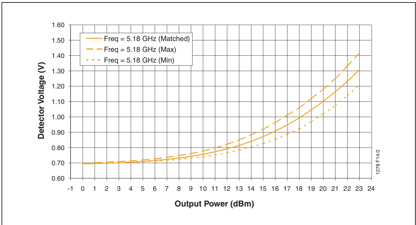
FIGURE 15: Detector Characteristics at Room Temperature with 2:1 Output VSWR All Phases at 5.18 GHz
