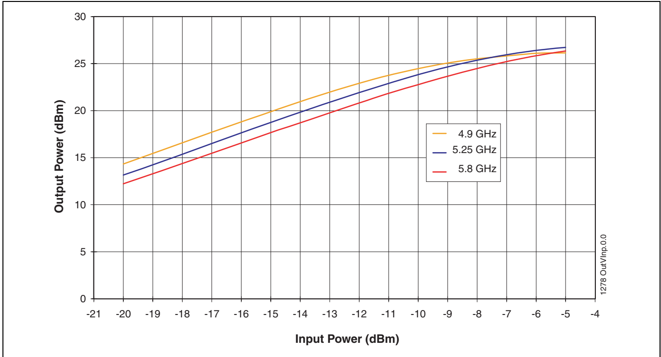
FIGURE 4: Output Power versus Input Power
