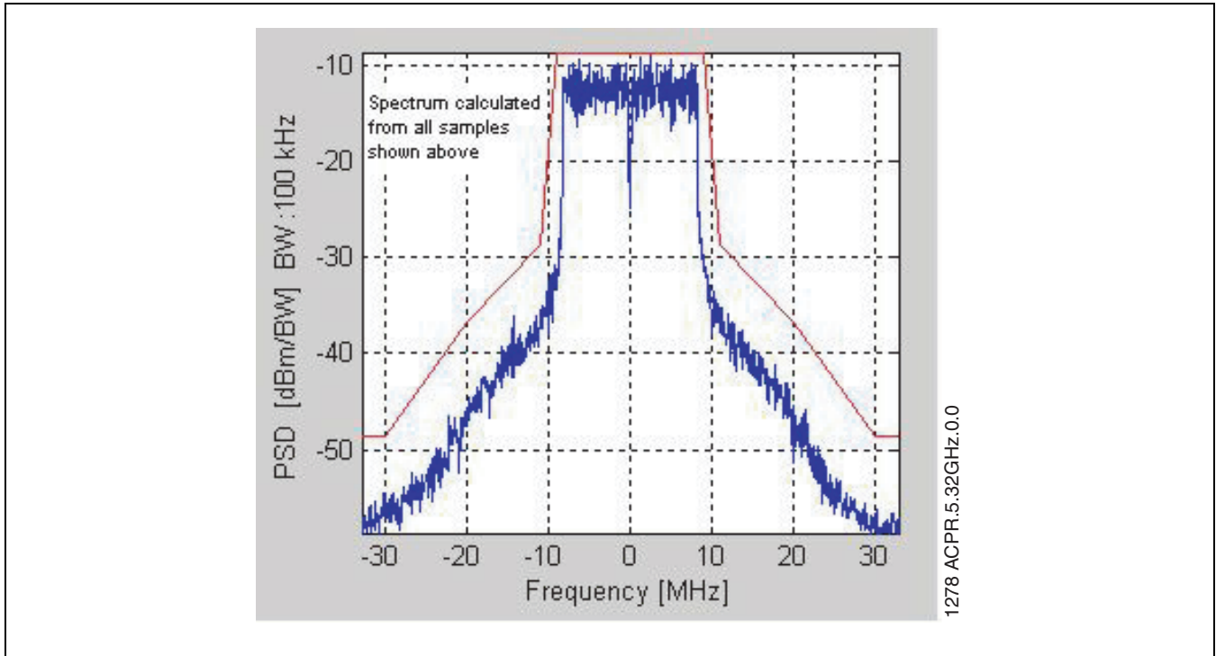
FIGURE 10: Frequency = 5.32 GHz at P_{OUT} = 23.5 dBm with I_{CC} = 385 mA
