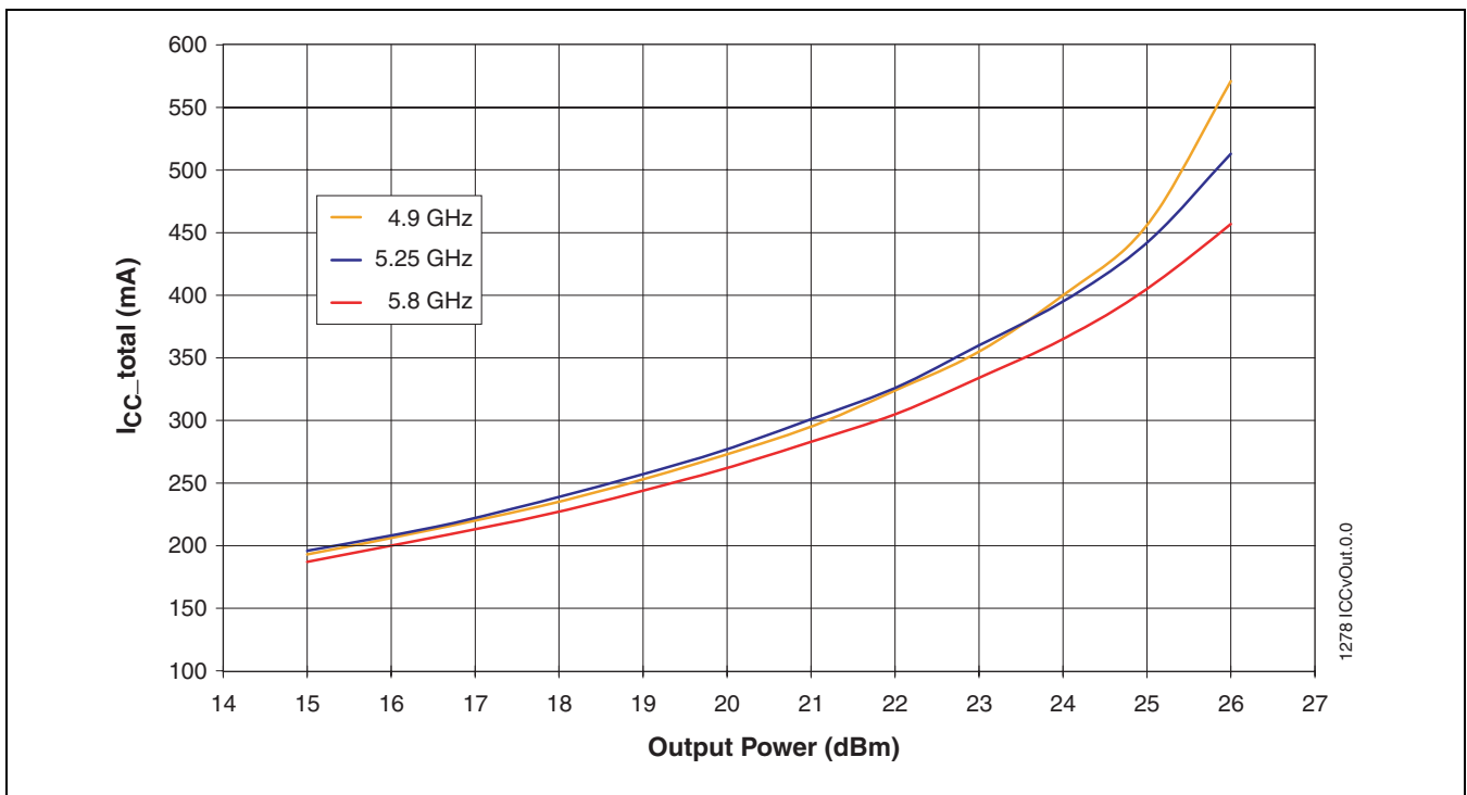
FIGURE 5: Power Supply Current versus Output Power
