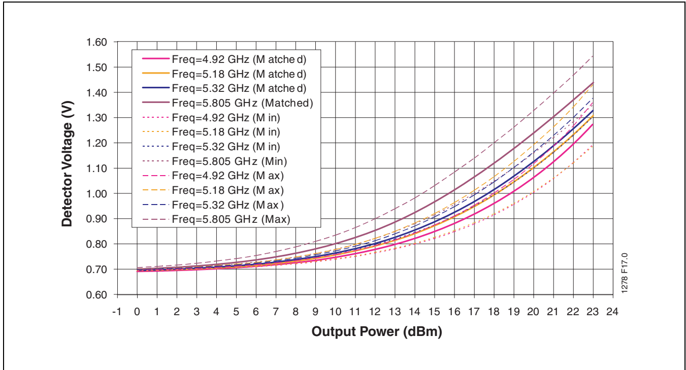
FIGURE 18: Detector Characteristics at Room Temperature Over Frequency with 2:1 Output VSWR All Phases
