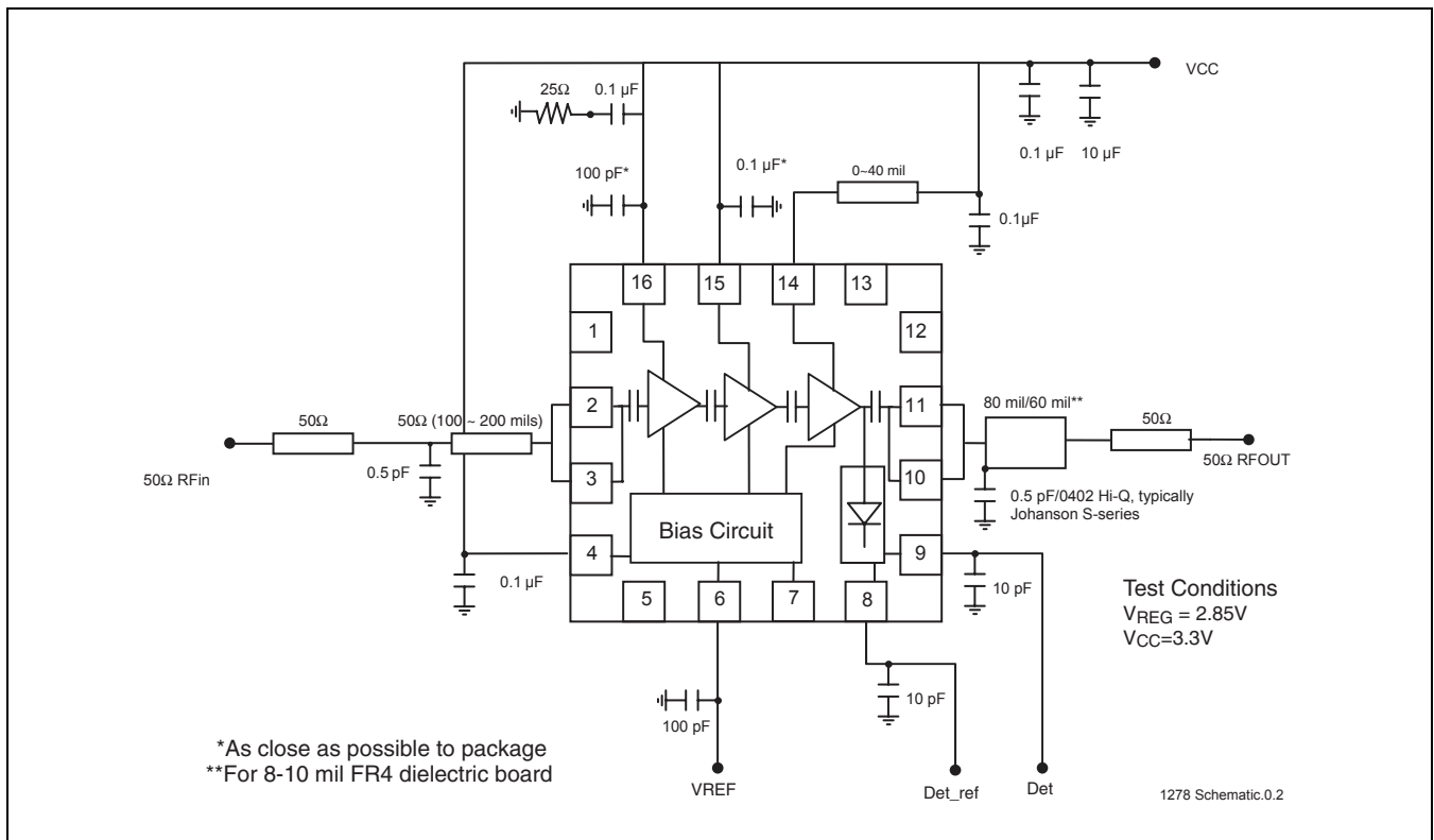
FIGURE 19: Typical Application for High-Power 802.11a Application
