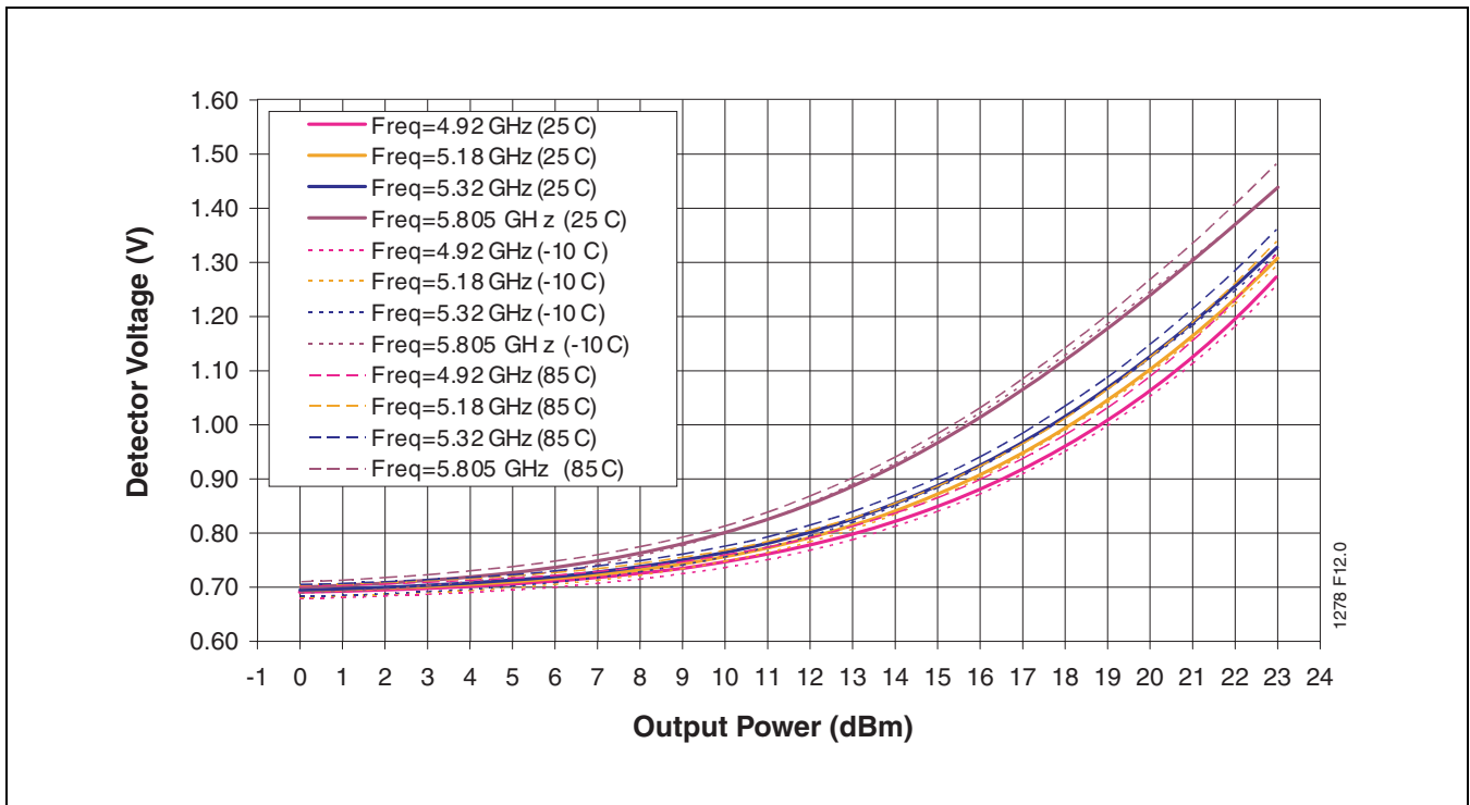
FIGURE 13: Detector Characteristics Over Temperature and Frequency
