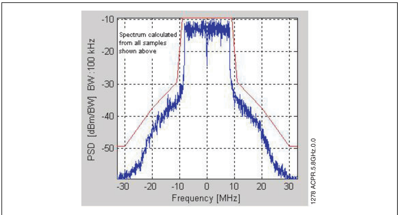
FIGURE 11: Frequency = 5.8 GHz at P_{OUT} = 23.5 dBm with I_{CC} = 365 mA
