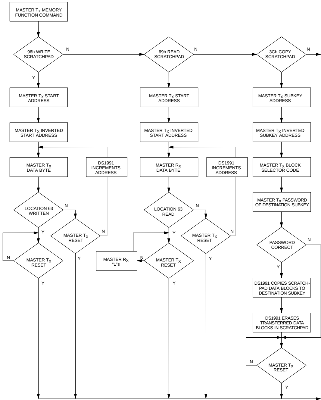
MEMORY FUNCTIONS FLOW CHART Figure 5
