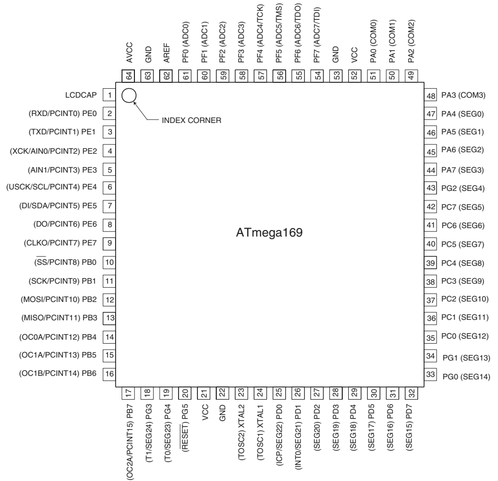
Figure 1. Pinout ATmega169
