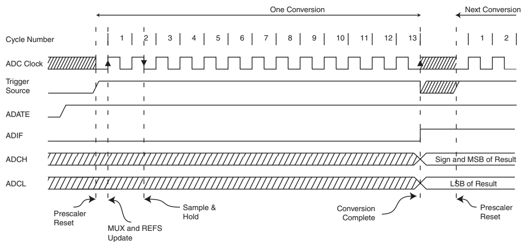
Figure 87. ADC Timing Diagram, Auto Triggerred Conversion
