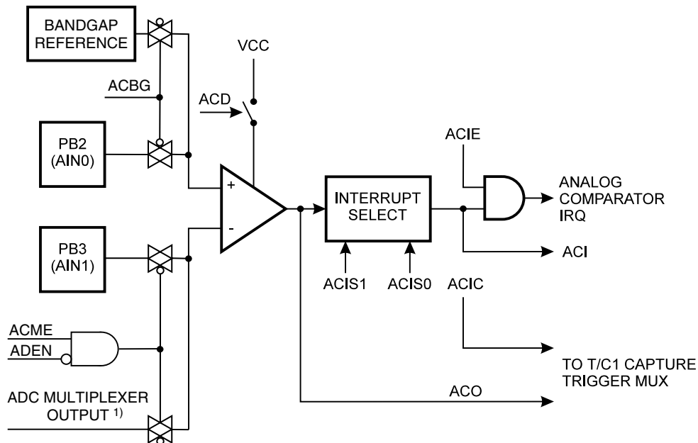
Figure 56. Analog Comparator Block Diagram
