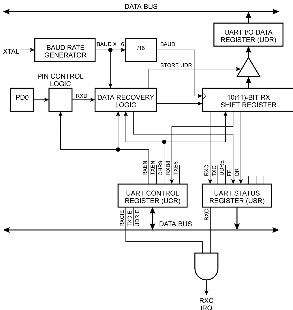
Figure 46. UART Receiver
