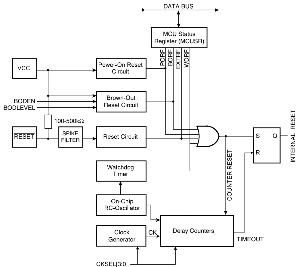
Figure 24. Reset Logic
