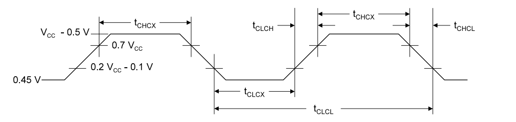
Figure 89. External Clock Drive Waveforms
