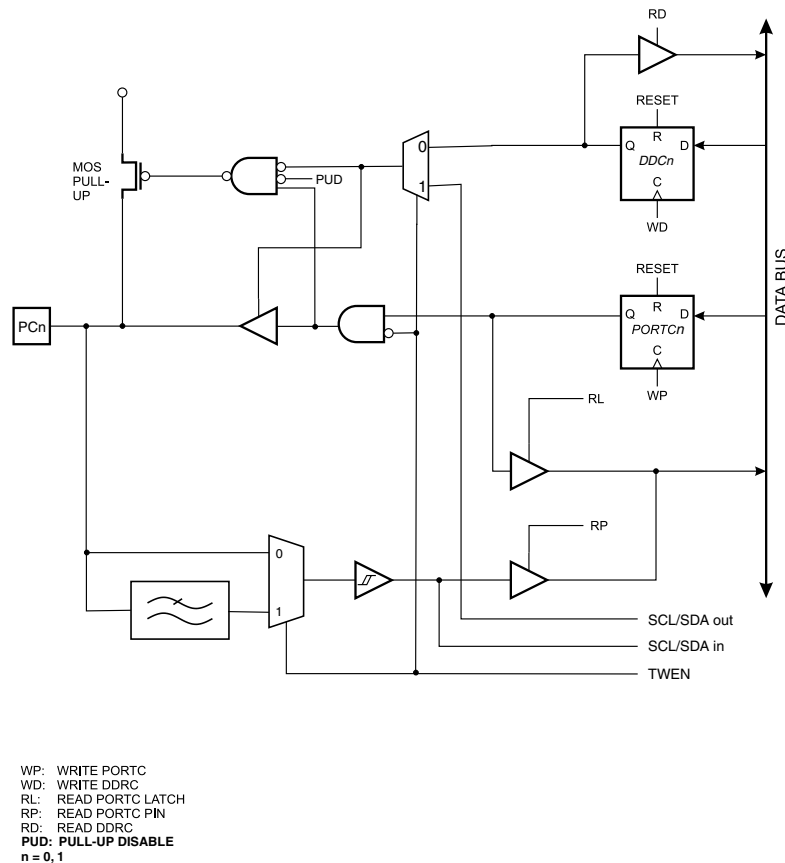
Figure 70. PORTC Schematic Diagram (Pins PC0 - PC1)
