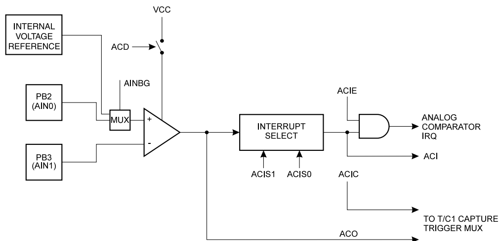
Figure 49. Analog Comparator Block Diagram
