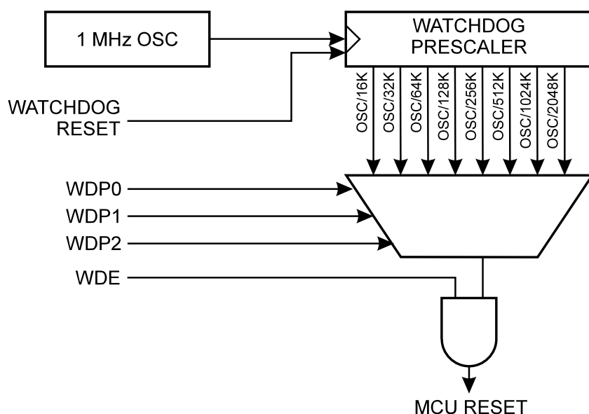
Figure 40. Watchdog Timer
