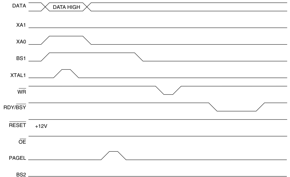
Figure 78. Programming the Flash Waveforms (Continued)
