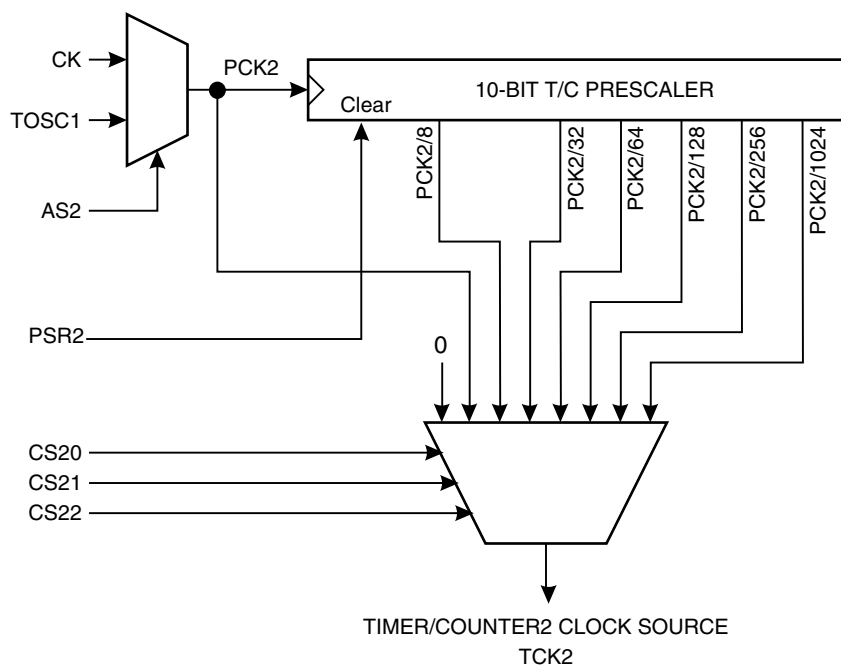
Figure 31. Timer/Counter2 Prescaler
