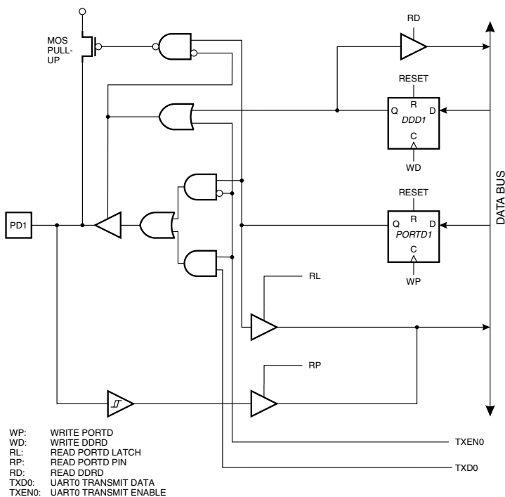
Figure 66. Port D Schematic Diagram (Pin PD1)
