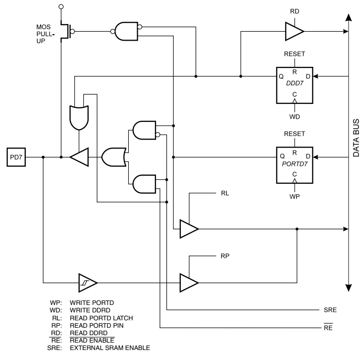
Figure 71. Port D Schematic Diagram (Pin PD7)
