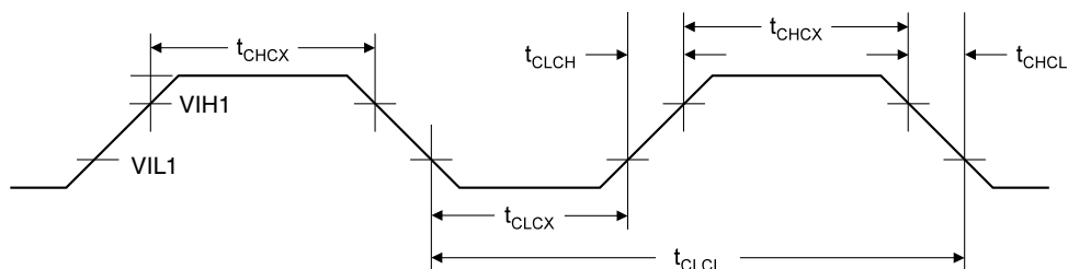
Figure 83. External Clock
