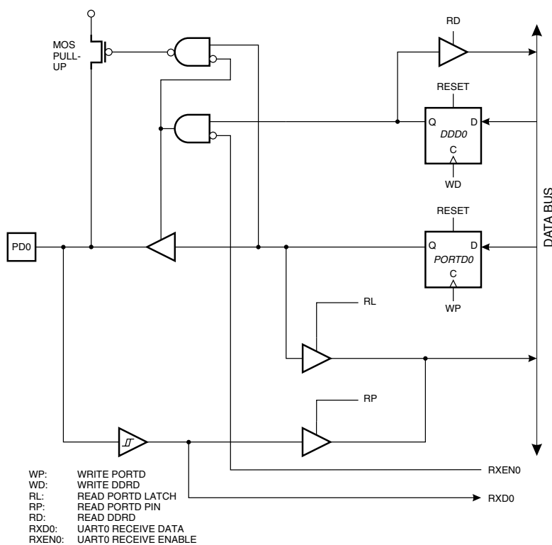
Figure 65. Port D Schematic Diagram (Pin PD0)
