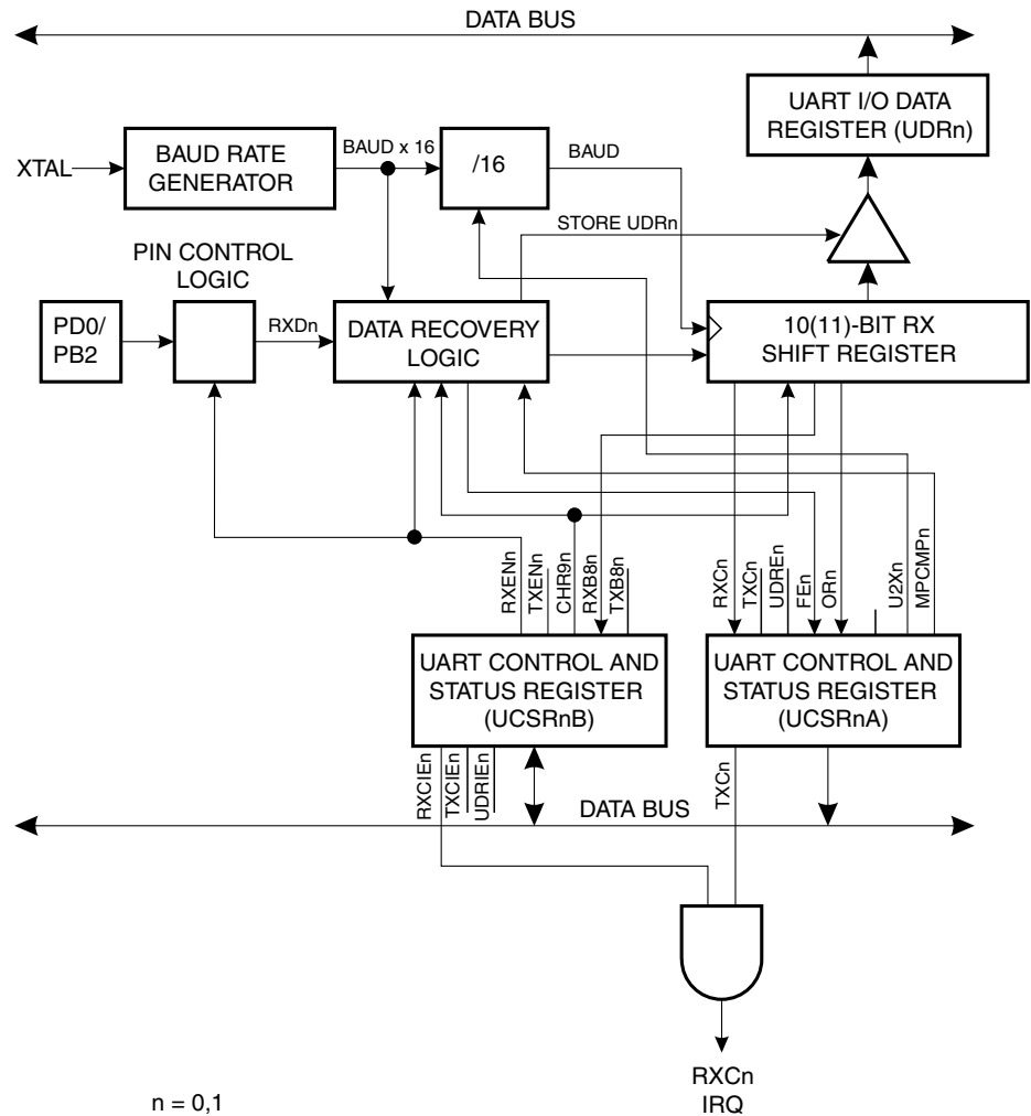
Figure 46. UART Receiver
