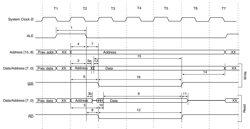
Figure 87. External Memory Timing (SRWn1 = 1, SRWn0 = 1) (1)
