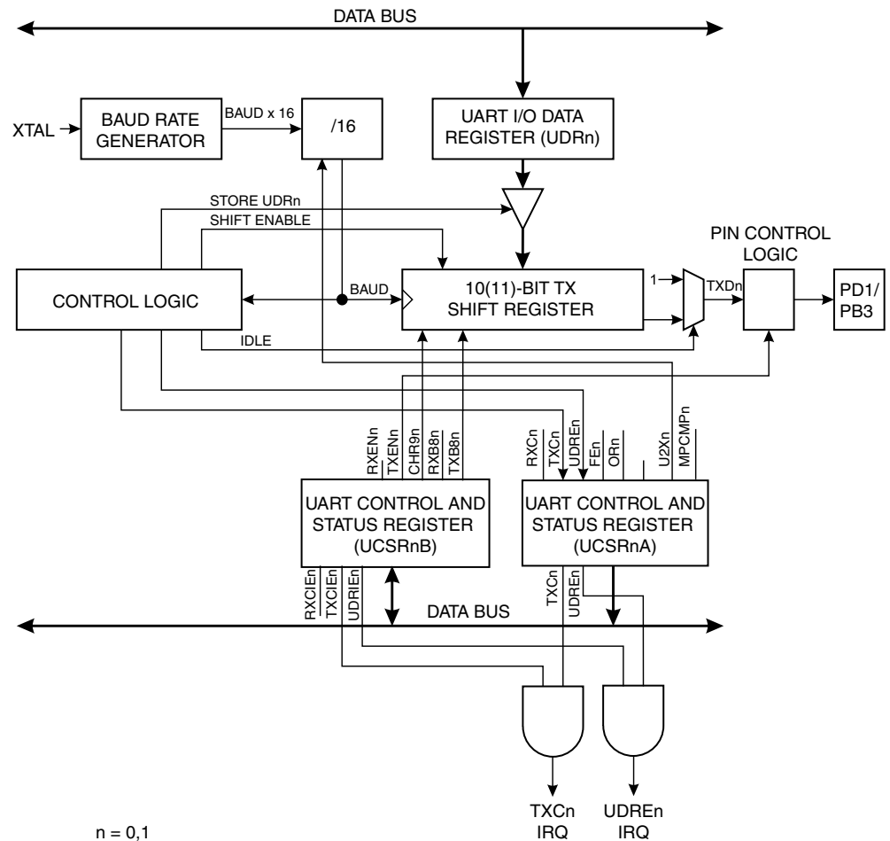
Figure 45. UART Transmitter
